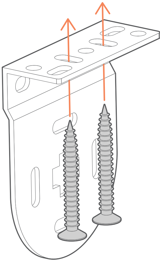
Top fixing Screw the brackets into the top of the recess.
