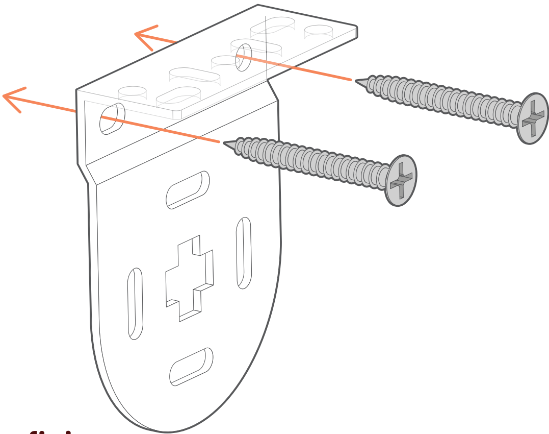
Side fixing Screw the brackets into the side walls of the recess.
