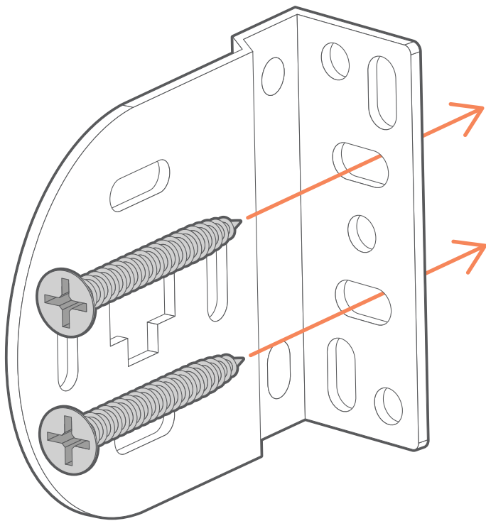
Face fixing Screw the brackets into the wall above the recess.
